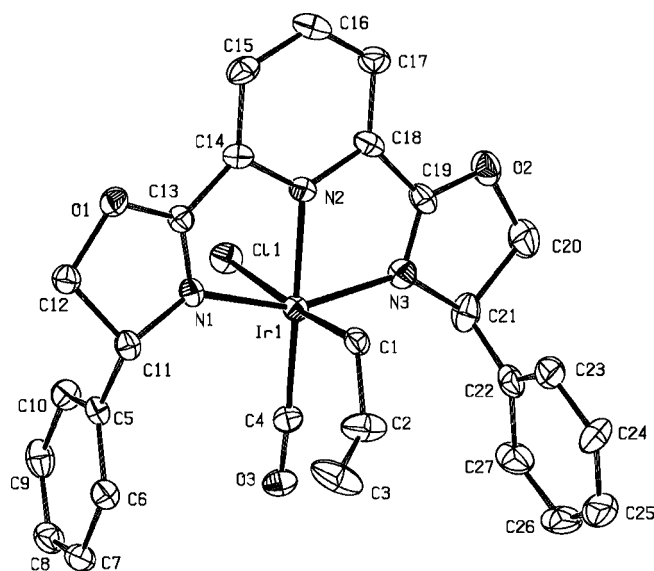
Figure 2. ORTEP-type view of the molecular structure of the cation of [\text{IrCl}(\eta^1\text{-CH}_2\text{CH=CH}_2)(\text{CO})\{\kappa^3\text{-}N,N,N\text{-}(S,S)\text{-}i\text{Pr-pybox}\}][\text{PF}_6] ( 15 ) drawn at the 10% probability level. Hydrogen atoms have been omitted for clarity.
