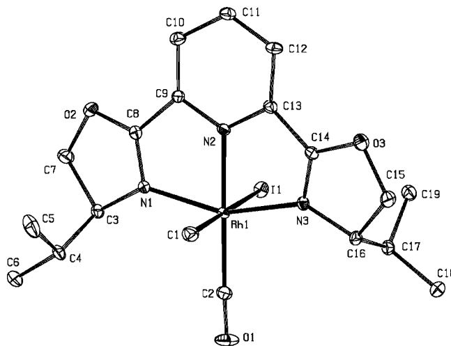
Figure 1. ORTEP-type view of the molecular structure of the cation of [\text{RhI}(\text{CH}_3)(\text{CO})(\kappa^3\text{-}N,N,N\text{-}(S,S)\text{-}i\text{Pr-pybox})][\text{PF}_6] ( 10 ) drawn at the 10% probability level. Hydrogen atoms have been omitted for clarity. Selected bond lengths [ \text{\AA} ] and angles [ ^\circ ]: Rh–N(1) 2.059(5), Rh–N(2) 1.994(5), Rh–N(3) 2.056(5), Rh–C(1) 2.120(8), Rh–C(2) 1.900(7), Rh–I 2.7759(14), C(2)–O(1) 1.113(10); N(3)–Rh–N(1) 156.5(2).
